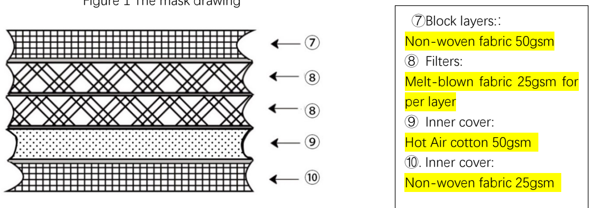
Figure 1 The mask drawing
