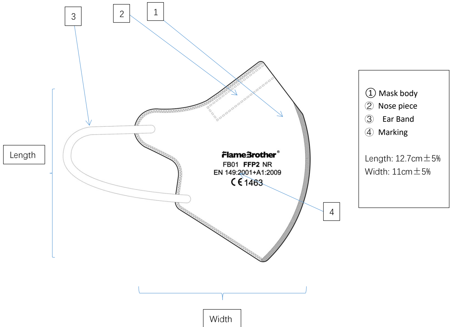
Figure 1 The mask drawing
